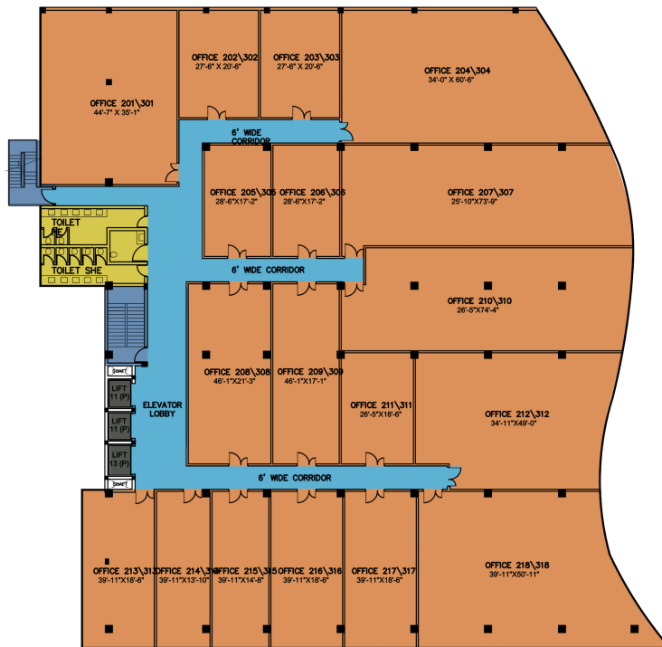
SECOND & THIRD FLOOR (TYPICAL)
